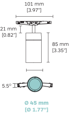
Flexible adaptor for curved track
