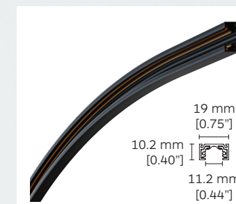
Horizontal curved track
