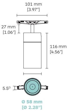
Flexible adaptor for curved track
