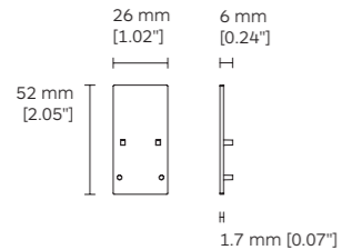
9219 End Cap with hole (For 2ST2)
