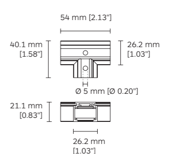
9255 T Type Joint Cover (For 2ST1)
