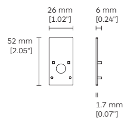
9219 End Cap with hole (For 2ST2)
