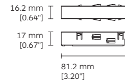
9292 Short Jointing Connector Non Polarized
