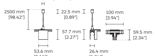
9255 T Type Joint Cover (For 2ST1)
