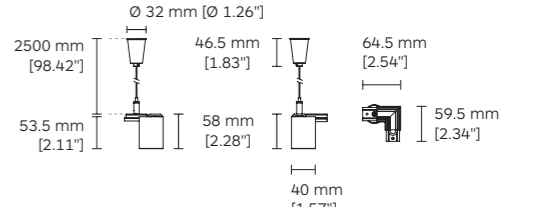
9254 T Joint cover with pendant wire (For 2ST2)
