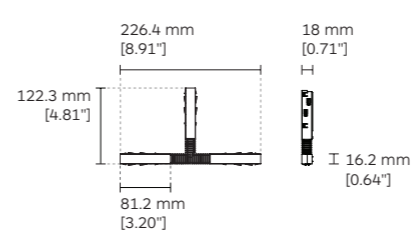
9249 T Jointing connector non polarized version
