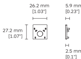
9222 End Cap with hole (For 2ST6)
