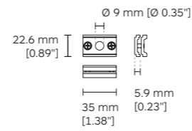
2H20 Straight connector (For 2ST2, 2ST6, 2ST7 & 2ST9)
