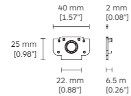
9220 End Cap (For 2ST3)
