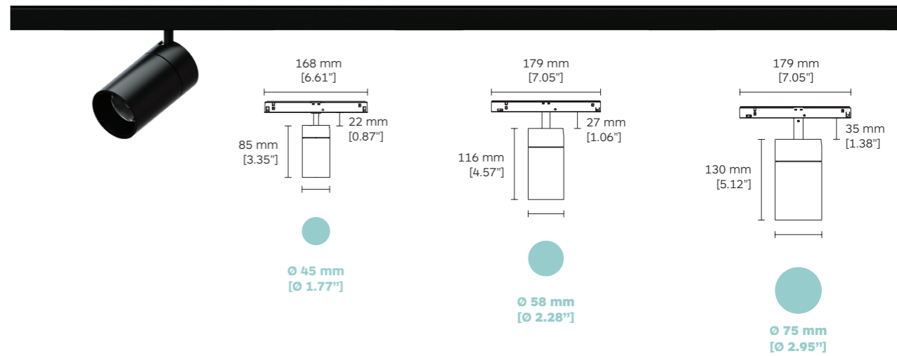
Regular Arm + Regular Track
