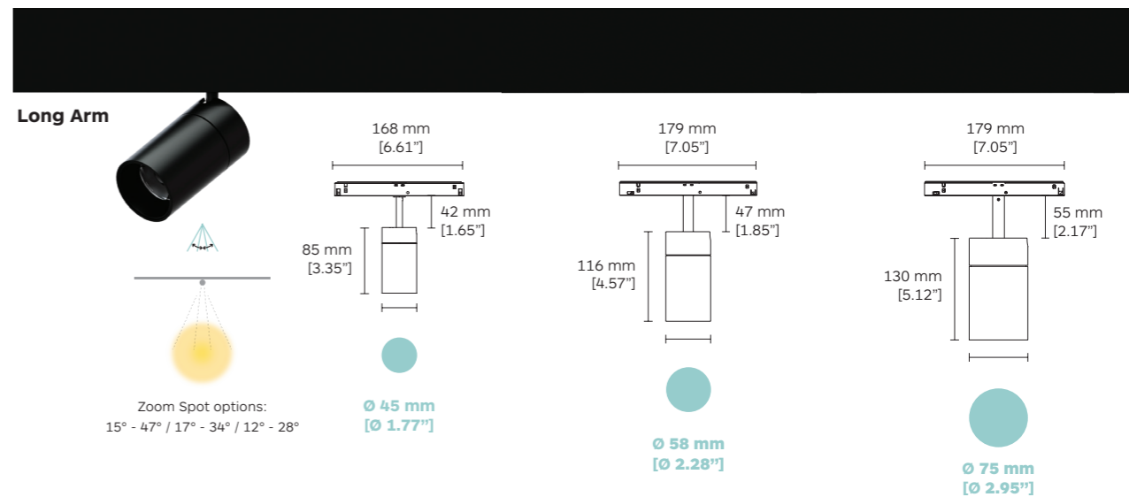
Long Arm + Deep Track
