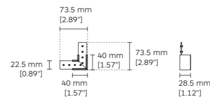
9234 Bracket for jointing connector (For 2ST2, 2ST6 & 2ST8)
