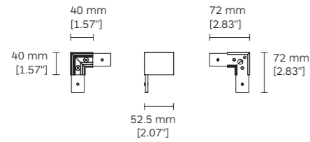
9215 L Bracket for angles (For 2ST2, 2ST6)
