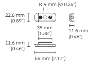
2H20 Straight connector (For 2ST2, 2ST6, 2ST7 & 2ST9)
