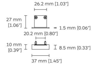
9224 End Cap (For 2ST9)
