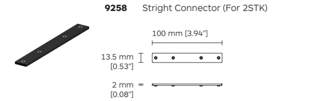
9258 Straight Connector (For 2STK)
