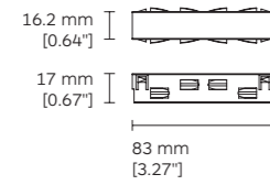
2G45N Narrow width cover
