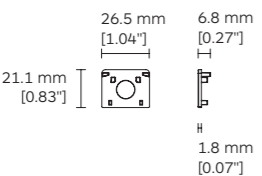
9218 End Cap (For 2ST2)
