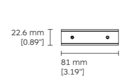
9234 Bracket for jointing connector (For 2ST2, 2ST6 & 2ST8)
