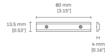
9230 End Cap (For 2ST7)
