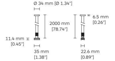
9252 Straight connector with pendant wire (For 2ST2, 2ST6, 2ST7 & 2ST9)
