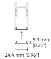
2G45M Medium width cover (For 2ST2, 2ST5, 2ST9, 2STA & 2STK)
