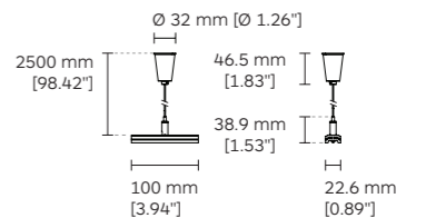
9253 L Joint cover with pendant wire (For 2ST2)
