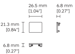
9217 End Cap with Hole (For 2ST1)
