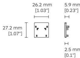
9221 End Cap (For 2ST6)
