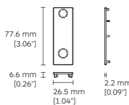
9225 Clamp (For 2ST2 & 2ST6)
